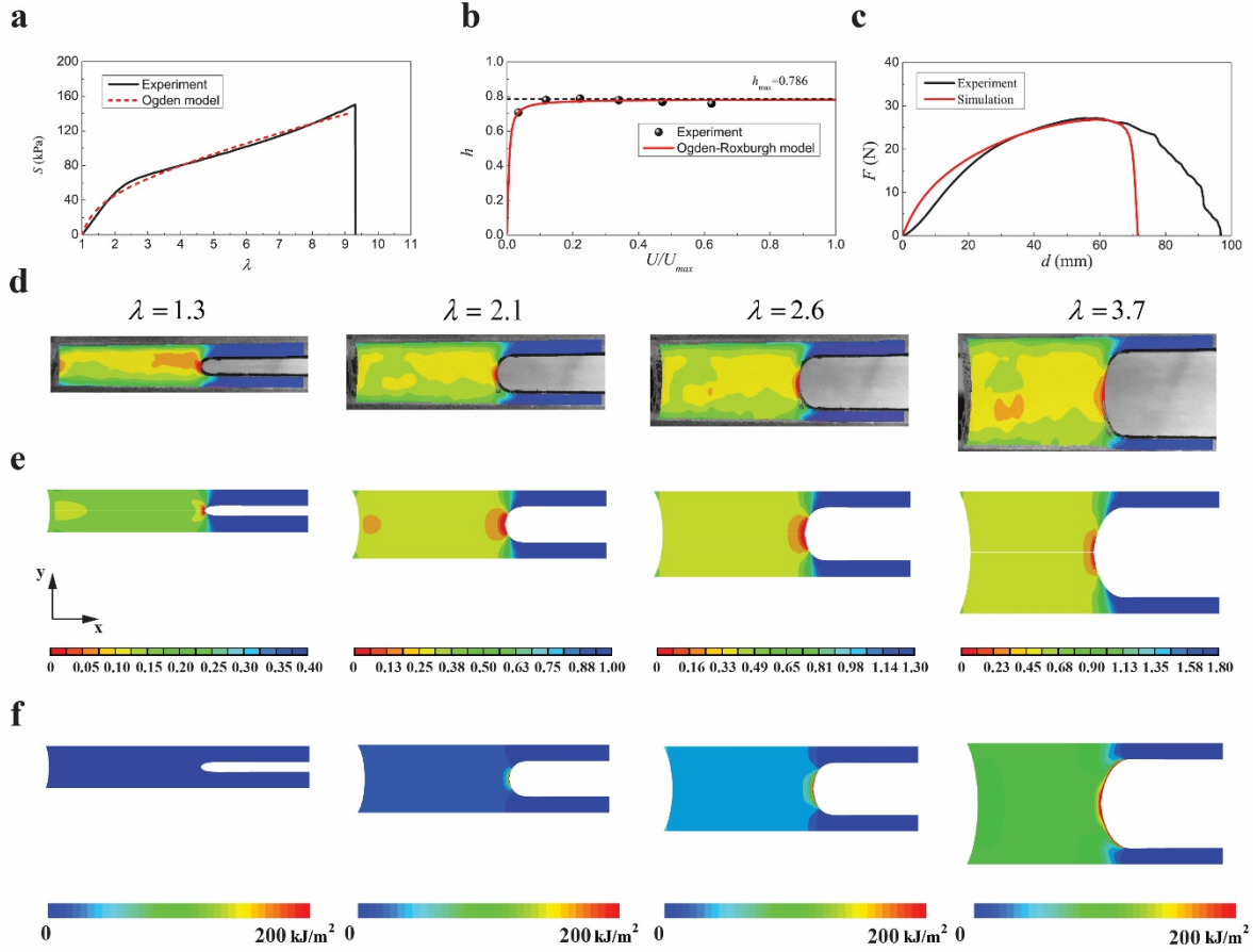
Figure S5. Comparison between experiments and simulations on fracture of PAAm-alginate hydrogel Sample 2. (a) Stress-stretch curves of the sample under pure-shear tensile deformation and one term Ogden model, i.e., \tilde{W} = 2\mu/\alpha_1^2 (\lambda_1^{\alpha_1} + \lambda_2^{\alpha_1} + \lambda_3^{\alpha_1} - 3) , with \mu = 26.49 kPa and \alpha_1 = 1.674 . (b) The measured hysteresis ratios of the material deformed to different stretches, and the calculated hysteresis ratio by the modified Ogden-Roxburgh model with r=1.203 and m=4.119 J/m 3 . (c) Force-displacement curves of the notched sample under pure-shear test
