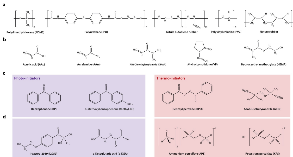
Figure S5. Reagents in hydrogel skin preparation. a-d) Chemical structures of diverse (a) polymers, (b) hydrogel monomers, (c) hydrophobic initiators, and (d) hydrophilic initiators for hydrogel skin preparation.
