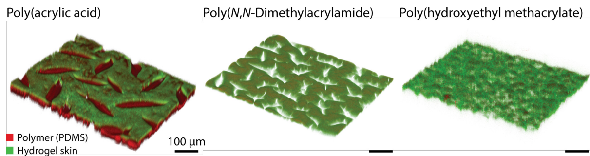
Figure S7. Confocal microscope images of hydrogel skins on PDMS substrates based various hydrogel monomers. PDMS and hydrogel skins are colorized by Nile red and fluorescein, respectively.
