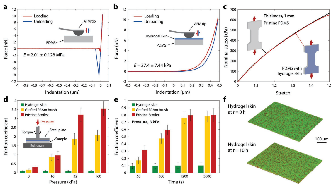
Figure 3. Mechanical properties of hydrogel skins. a,b) Nanoindentation curves for PDMS substrates without (a) and with (b) hydrogel skins. Values for Young's modulus indicate the average and the standard deviation ( n = 20 repeats). c) Nominal stress versus stretch curves for PDMS substrates with and without hydrogel skins. d) Friction coefficients of pristine Ecoflex, Ecoflex grafted with PAAm brush, and Ecoflex with hydrogel skins under different normal pressures ( n = 3 repeats). e) Friction coefficients of pristine Ecoflex, Ecoflex grafted with PAAm brush, and Ecoflex 30 with hydrogel skins at 3 kPa normal pressure after the extended periods of friction testing ( n = 3 repeats). f) Confocal microscopy images of hydrogel skins before and after 10 h friction testing. Ecoflex and hydrogel skins are colored by Nile red and fluorescein, respectively.
