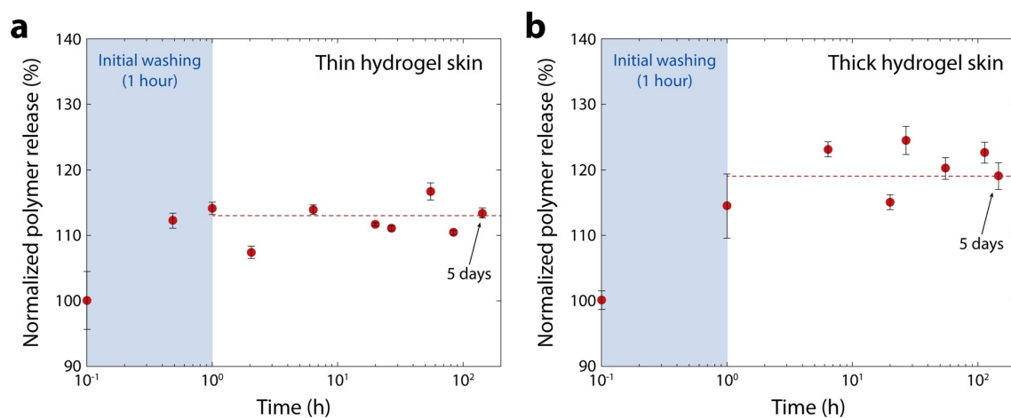
Figure S2. Leaching of unreacted reagents from hydrogel skins. a,b) Normalized polyacrylic acid monomer and polymer release over time for (a) thin and (b) thick hydrogel skins on PDMS substrates ( n = 3 repeated).
