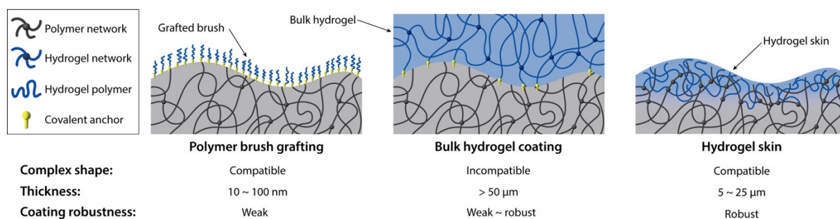
Figure S1. Comparison between polymer brush grafting, bulk hydrogel coating, and hydrogel skin in terms of compatibility to complex shapes, thickness, and robustness of coatings.
