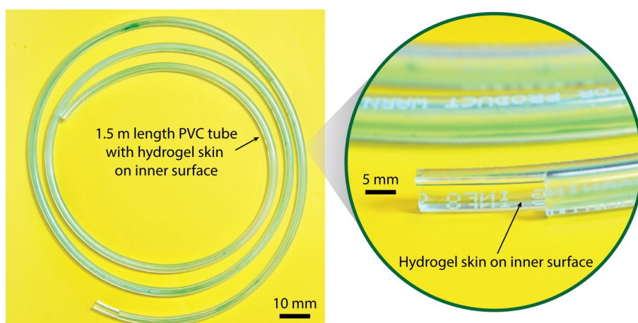
Figure S11. Long PVC tubing with lumen uniformly coated with hydrogel skin. Hydrogel skins are colorized by green food dye.
