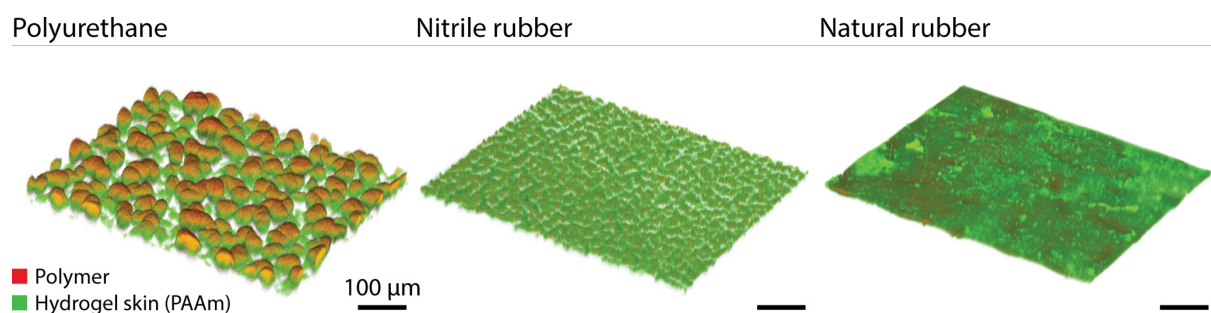
Figure S6. Confocal microscope images of hydrogel skins on various polymer substrates based on AAm. Polymers and hydrogel skins are colorized by Nile red and fluorescein, respectively.
