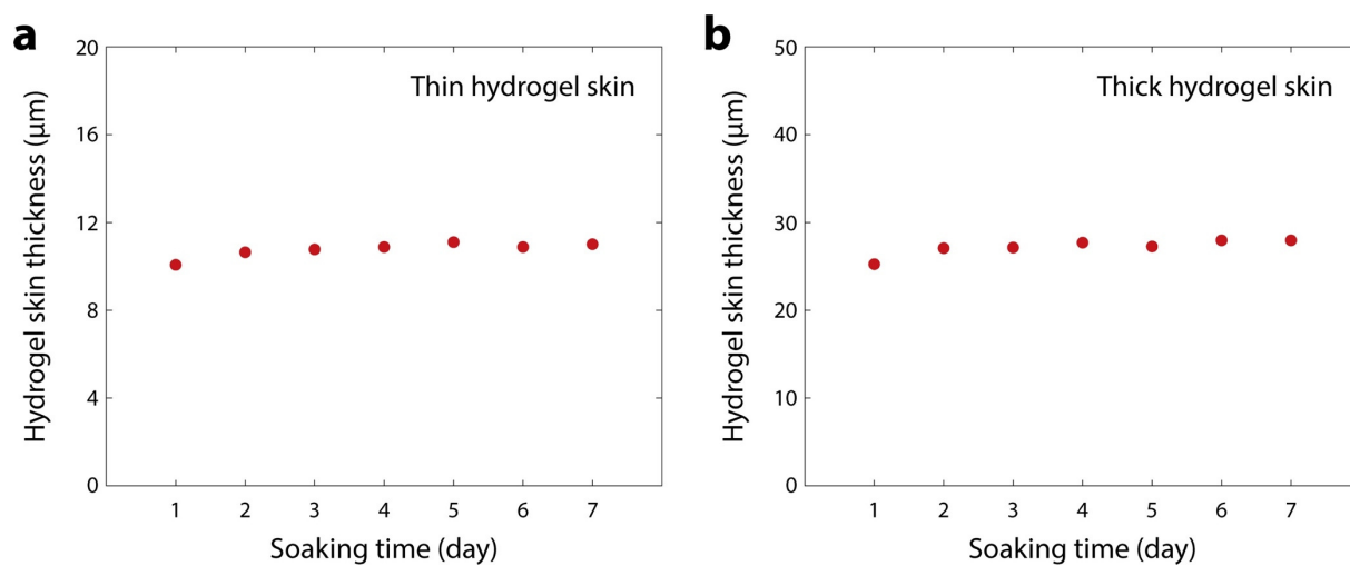
Figure S4. Change in thickness of the hydrogel skins over time in aqueous environment. a,b) The thickness of AAm-based (a) thin and (b) thick hydrogel skins on PDMS substrates over time soaked in water.
