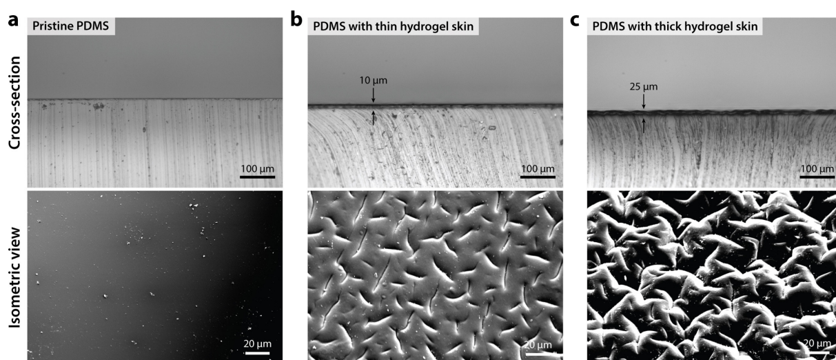
Figure S3. Cross-section and surface images of hydrogel skins. a-c) Microscope images for cross-section and SEM images for surfaces of (a) pristine PDMS, (b) PDMS with thin hydrogel skins, and (c) PDMS with thick hydrogel skins.
